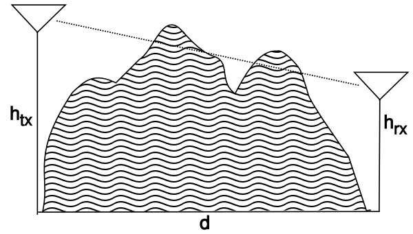
Fig. 6. Schematic of link geometry used by terrain models.
